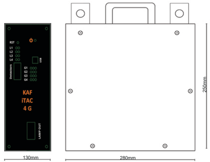
EXTERNAL VIEW
